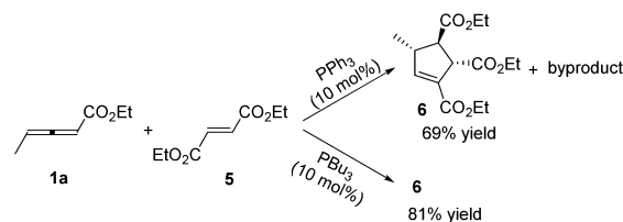
Scheme 2 Phosphine-catalysed (3+2) cycloaddition reactions of acrylate, vinyl phenyl sulfone or fumarate with \gamma -methyl allenates.
