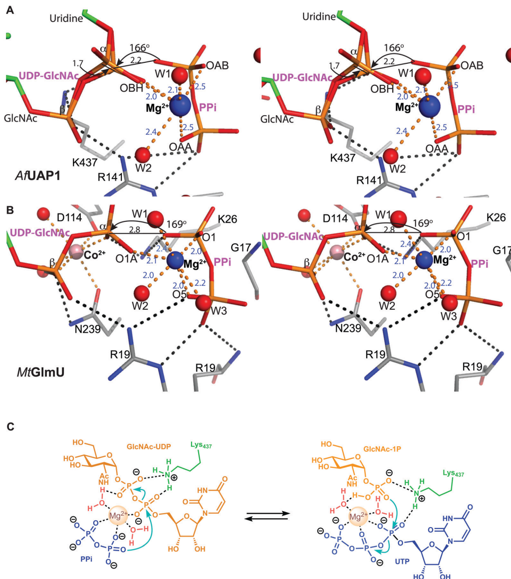
Fig. 5 Magnesium coordination and AfUAP1 mechanism. (A) Magnesium coordination in the AfUAP1 -UDP-GlcNAc-Pi-Mg 2+ complex active site. A view of the active site of the AfUAP1 -UDP-GlcNAc-Pi-Mg 2+ and MtGlmU -UDP-GlcNAc-Pi-Mg 2+ -Co 2+ complexes. The attack distance for pyrophosphorolysis is 2.2 and 2.8 Å and the attack angle is 166° and 169° for UAP1 and GlmU, respectively. The distance between the α-phosphates in both UDP-GlcNAc adopting the dual conformation is 1.7 Å. The Mg 2+ is tetragonal bipyramidally coordinated (albeit with a disordered 6th ligand in AfUAP1 ) as suggested by coordination distances and angles. (B) Magnesium coordination in the MtGlmU -UDP-GlcNAc-Pi-Mg 2+ -Co 2+ complex active site. (C) Schematic diagram of the proposed forward and reverse reaction mechanisms. The left panel indicates chemical bond formation/cleavage (cyan arrows) in the AfUAP1 -Ppi-UDP-GlcNAc ternary complex shown in Fig. 5A leading to the formation of GlcNAc-1P and UTP. The right panel using the same ternary complex structure as a template indicates chemical bond formation/cleavage in the reverse reaction leading to the formation of UDP-GlcNAc and Ppi from GlcNAc-1P and UTP is proposed.
