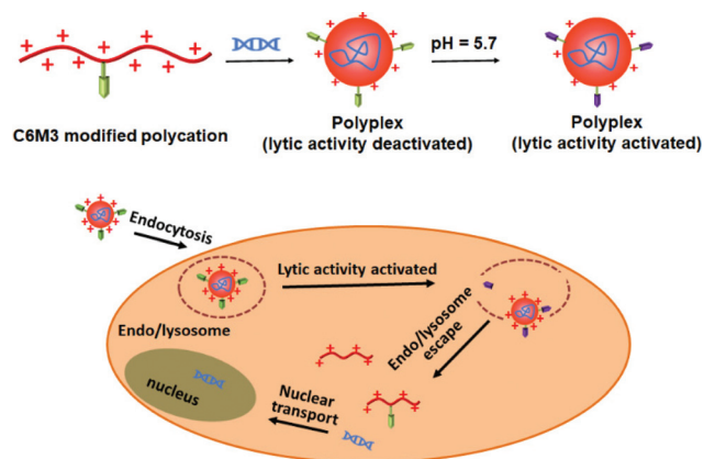
Scheme 1 Illustration of C6M3 modified polycations for successful gene delivery.
