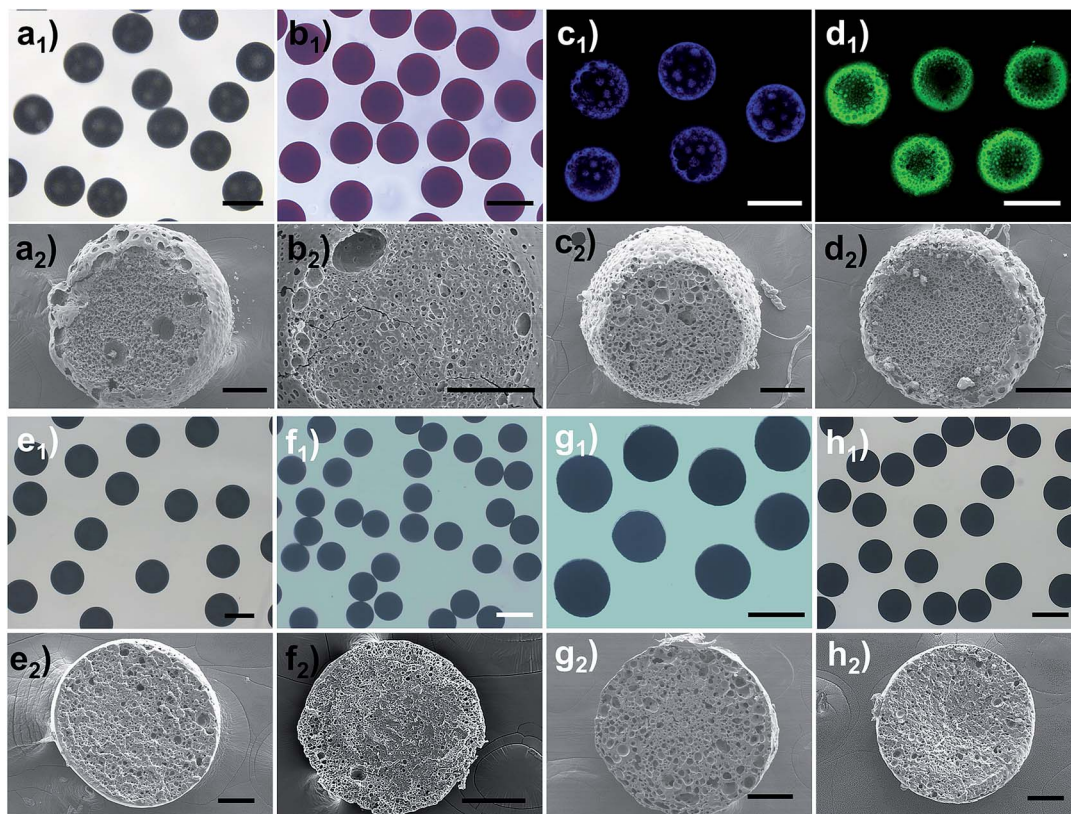
Fig. 8 Great extensibility of our proposed osmotically driven phase separation. Optical and SEM images of the formed pore-structured spheres by using C_{36}\text{vim}[\text{Tf}_2\text{N}]-\text{LiTf}_2\text{N} as a general phase separation carrier platform for realizing the phase separation of various substances: (a 1–2 ) ETPTA, (b 1–2 ) azobenzene-type monomer, (c 1–2 ) AIE-type monomer, (d 1–2 ) bioorthogonal monomer (click reaction with GOX-FITC enzyme), (e 1–2 ) \text{TiO}_2 particles, (f 1–2 ) Au nanoparticles, (g 1–2 ) carbon nanotubes, and (h 1–2 ) graphene. Scale bars are 400 \mu\text{m} (a 1–h 1 ) and 100 \mu\text{m} (a 2–h 2 ).
