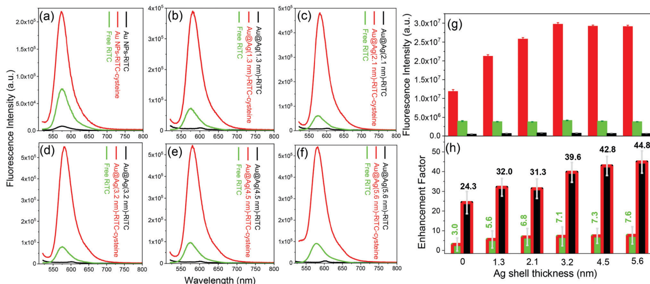
Fig. 4 (a)–(f) Fluorescence spectra of free RiTC (green), isolated metal–RiTC NPs (black) and optimum coupled metal–RiTC NPs (red) with different Ag shell thicknesses (0, 1.3, 2.1, 3.2, 4.5, and 5.6 nm). (g) The corresponding fluorescence intensity of optimum coupled Au@Ag–RiTC NPs (red bar), free RiTC (green bar) and isolated Au@Ag–RiTC NPs (black bar). (h) Enhancement factor versus free RiTC ( I_{\text{coupled metal-RiTC NPs}}/I_{\text{free RiTC}} , green bar) and enhancement factor versus pre-quenched RiTC ( I_{\text{coupled metal-RiTC NPs}}/I_{\text{isolated metal-RiTC NPs}} , black bar) for different Au@Ag NPs.
