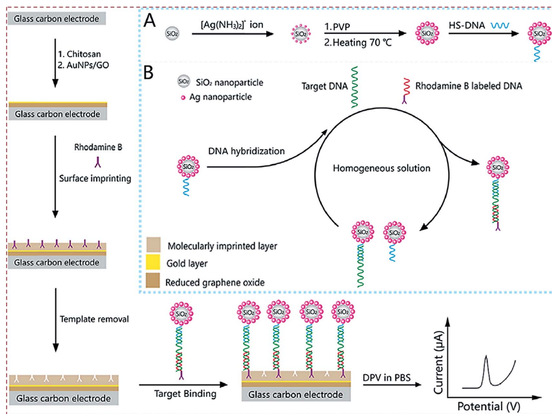
Fig. 19 Schematic illustration of a MIP-based electrochemical DNA biosensor for the determination of breast cancer susceptibility gene (BRCA-1) amplified by \text{SiO}_2/\text{Ag} . Insets of (A) and (B) show the preparation process of \text{SiO}_2/\text{Ag}/\text{DNA} and homogeneous DNA hybridization. Reproduced with permission from ref. 154. Copyright 2018, Elsevier.
