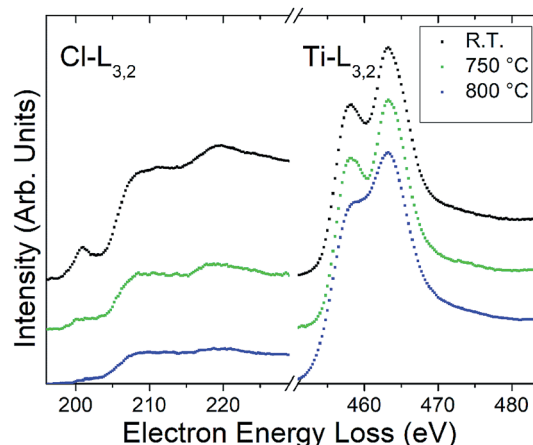
Fig. 4 Electron energy loss spectroscopy from a thin edge of a \text{Ti}_3\text{C}_2\text{Cl}_2 multilayer particle, showing the background subtracted and multiple scattering deconvolved Cl- and Ti- \text{L}_{3,2} edges under ambient conditions and after heating at 750 and 800^\circ\text{C} . The spectra are normalized against the Ti-L _2 peak maximum and vertically separated for clarity.
