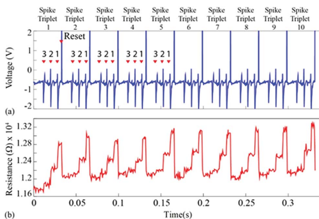
Fig. 4 (a) Input signal used for Fig. 3. Ten copies of a spike triplet were concatenated and fed to the device-under-test. The triplet was composed of the three average spike prototypes arranged in increasing order of amplitude i.e. order 3, 2, 1. Reset pulses followed every spike triplet. This stimulus was chosen in order to experimentally demonstrate the response repeatability of the device-under-test. (b) Resistive state evolution of the device in response to the neural recording in (a).
