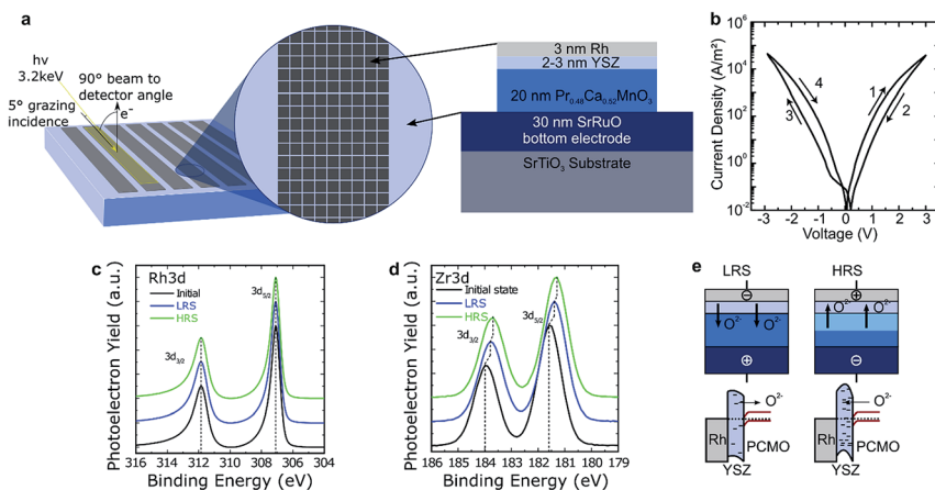
Fig. 1 (a) Sketch of the sample layout of PCMO/YSZ devices with a side length of 50 \mu\text{m} and the geometry for HAXPES measurements with an illustration of the layer stack. The devices consist of Rh/YSZ/PCMO which is etched away outside the device area down to the SRO bottom electrode. (b) I - V curve of one PCMO/YSZ device. (c) and (d) show spectra for the core-levels of (c) Rh 3d and (d) Zr 3d for the initial, high and low resistive states, respectively. The photon energy was set to 3.2 keV. A Shirley background was subtracted from the data and they were normalized to the maximum intensity to allow for easier comparison of the line shapes and the peak positions. (e) Sketch of the movement of oxygen in the PCMO/YSZ stack with electrical biasing and corresponding change of the energy bands at the interface.
