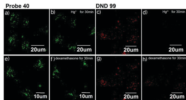
Fig. 60 Fluorescence images of MCF-7 cells stained with probe 40 (pseudo green) and DND-99 (pseudo red) stimulated with 100 \mu M \text{Hg}^{2+} [(a and b) probe 40 ; (c and d) DND-99] and 10 \mu M dexamethasone [(e and f) probe 40 ; (g and h) DND-99]. Copyright 2014 American Chemical Society.
