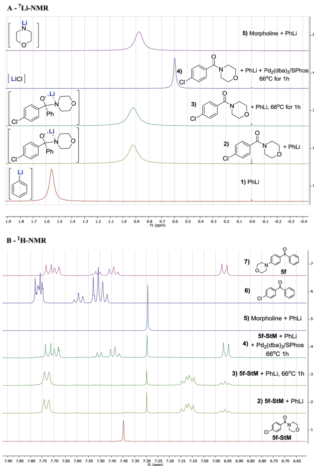
Fig. 1 ^7Li (A) and ^1H (B)-NMR analysis of the reaction with (4-chlorophenyl)(morpholino)methanone. Conditions: 0.1 mmol in 0.7 mL of THF- d_8 at 25 °C with LiCl in D_2O as internal standard. Hypothesized structure of lithium species between brackets.
