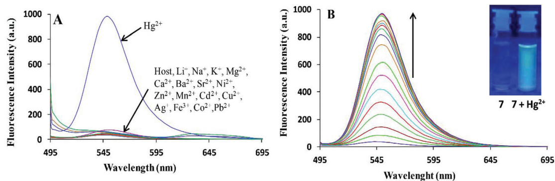
Fig. 13 (A) Changes in the fluorescence emission spectra of 195 nM solution of 12 (FON) upon the addition of 10 μM of different metal ion salts in 15 aqueous media; (B) changes in the fluorescence emission spectra of 195 nM solution of 12 (FON) upon the successive addition of 0 to 10 μM of \text{Hg}^{2+} in an aqueous medium. Adapted with permission from ref. 70. Copyright 2013 the Centre National de la Recherche Scientifique (CNRS) and the Royal Society of Chemistry.
