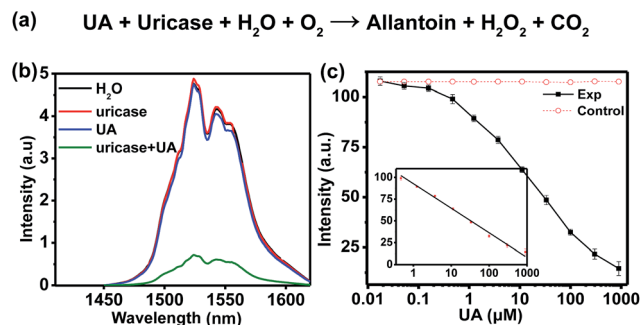
Fig. 4 (a) Chemical equation for the generation of \text{H}_2\text{O}_2 through UA/uricase reaction. (b) NIR-II emission spectra of \text{NaCeF}_4:\text{Er}/\text{Yb} NCs ( 0.5 \text{ mg mL}^{-1} ) after the addition of 100 \mu\text{L} of \text{H}_2\text{O} , uricase ( 0.011 \text{ U mL}^{-1} ), UA ( 900 \mu\text{M} ) and uricase ( 0.011 \text{ U mL}^{-1} ) + UA ( 900 \mu\text{M} ), respectively, upon excitation at 980 \text{ nm} . (c) Calibration curve for the UA assay. The control experiment was carried out by replacing UA with \text{H}_2\text{O} under otherwise identical conditions. The inset shows the linear range ( 0.411\text{--}900 \mu\text{M} ) of the calibration curve.
