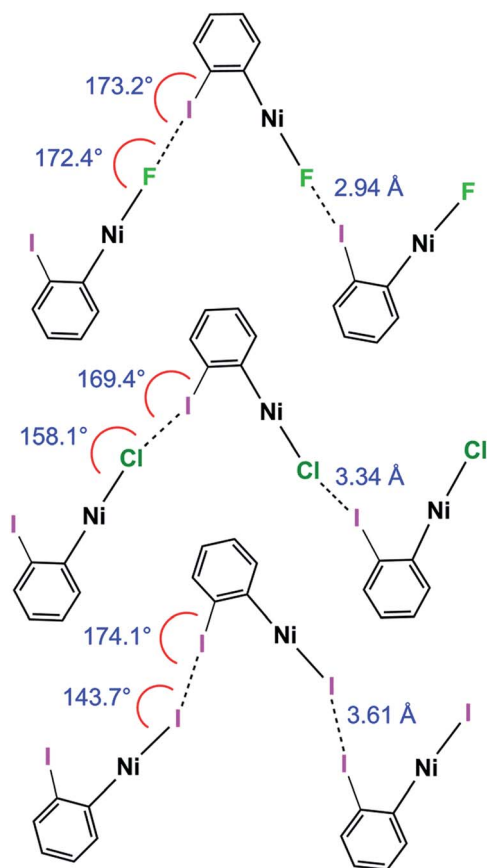
Scheme 6 Halogen bond length and C-I\cdots Ni and I\cdots X-Ni angles for 1oF , 1oCl and 1oI ( \alpha ) (phosphines and aromatic fluorines omitted, for esd's see Table 2).
