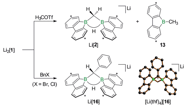
Scheme 11 The addition of \text{H}_3\text{C-I} to \text{Li}[2] furnishes the bis(9-borafluorenyl)methane 14^{\text{C1}} . Carbon atoms marked with asterisks bear t Bu substituents.
