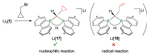
Scheme 10 The reactions of Yamashita's and Nozaki's boryllithium compound with \text{H}_3\text{COTf} or \text{BnBr} furnish the corresponding methyl borane or bromoborane, respectively (top). In the analogous reactions with \text{Li}_2[1] , only the organyl moieties are transferred to boron (middle; cf. \text{Li}[2]/13 and \text{Li}[16] ). The reaction of \text{Li}_2[1] with the radical clock (bromomethyl)cyclopropane quantitatively furnishes \text{Li}[17] , which is a strong indication for a closed-shell, nucleophilic pathway (bottom). \text{Dipp} = 2,6\text{-}(\text{iPr})_2\text{C}_6\text{H}_3 , \text{Bn} = \text{CH}_2\text{C}_6\text{H}_5 , \text{H}_3\text{COTf} = \text{H}_3\text{COSO}_2\text{CF}_3 ; carbon atoms marked with asterisks bear t Bu substituents. In the crystal structure plot of [\text{Li}(\text{thf})_4][16] , the solvent-separated cation, the t Bu groups, and all \text{C}(\text{sp}^2)\text{-H} atoms are omitted for clarity.
