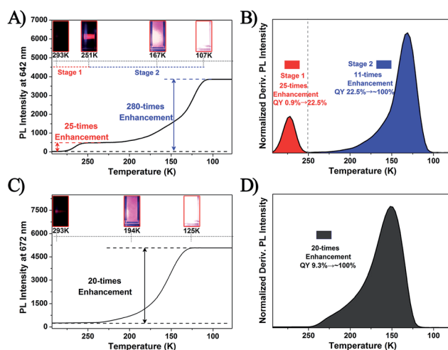
Fig. 6 The PL intensity at the fixed points of (A) 642 nm for the Ag_{29}(BDT)_{12}(TPP)_4 NC and (C) 672 nm for the Pt_1Ag_{28}(S-Adm)_{18}(TPP)_4 NC at different temperatures. Insets: the digital photographs of each NC in DMF solution under UV light. The derivative results for PL intensity of (B) Ag_{29}(BDT)_{12}(TPP)_4 and (D) Pt_1Ag_{28}(S-Adm)_{18}(TPP)_4 NCs.
