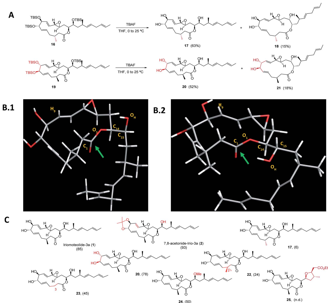
Scheme 2 (A) Final deprotection towards C_3 -irio-3a epimer ( 17 ) and C_7,C_8 -irio-3a diastereoisomer ( 20 ) in the presence of TBAF. (B) Blueprint of the most stable conformers for iriomoteolide-3a ( 1 , B.1) and its C_3 -epimer ( 17 , B.2). 1 : O_1-C_{14}-C_{15}-O_H = -63^\circ . 17 : O_1-C_{14}-C_{15}-O_H = +62^\circ . (C) Synthetic iriomoteolide derivatives using the general strategy reported in Scheme 1B and preliminary evaluation of their anti-proliferative activity. Values in brackets represent the % of growth inhibition of Daudi cells at 10 \mu M concentration of the compound. N.d.: not determined.
