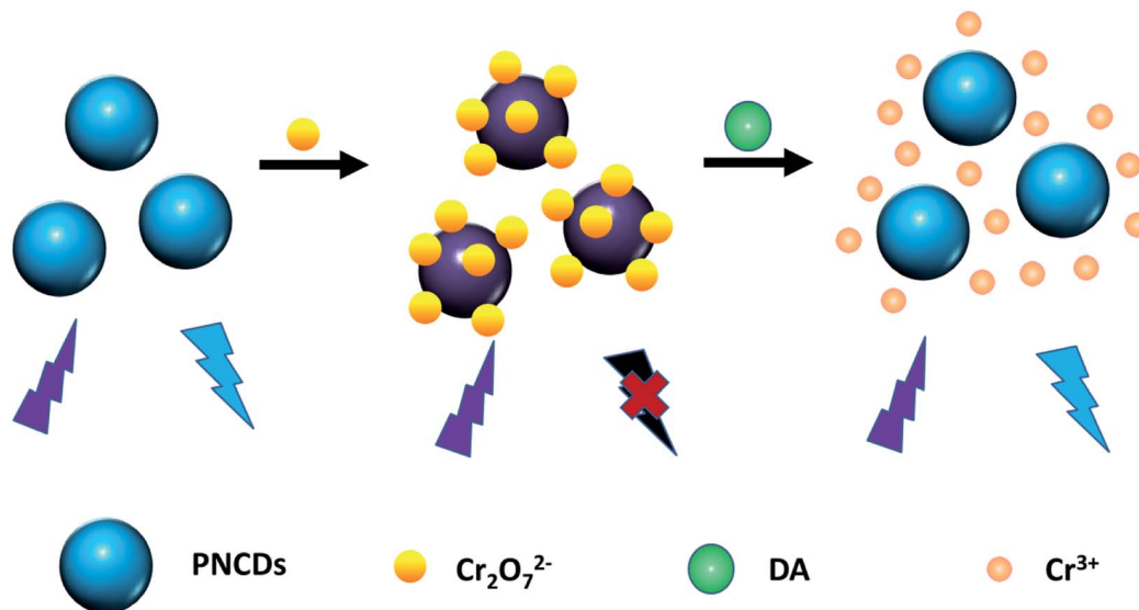
Scheme 1 Diagrammatical explanation of fluorescence mechanism for \text{Cr}(\text{vi}) and DA based on IFE of PNCDs.
