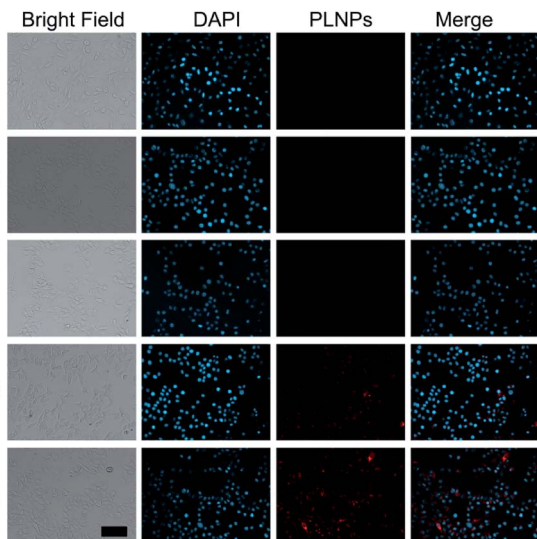
Fig. 6 Intracellular assay of PLNPs–CuS nanoparticles for 3T3 cells and HepG2 cells treated with different amounts (0 \mu\text{M} , 5 \mu\text{M} , 10 \mu\text{M} , and 20 \mu\text{M} ) of AFT B1. The scale bar represents 40 \mu\text{m} for all images.
