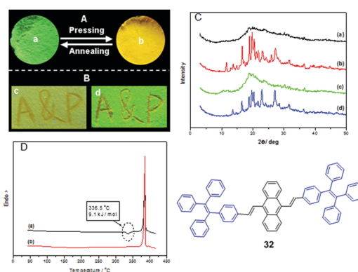
Fig. 6 The images of luminogen 32 taken at room temperature. (A) Annealed sample (a) and pressed sample (b) under 365 nm UV-light; (B) cast on filter paper after writing "A&P" with a metal spatula: (a) natural light and (b) 365 nm UV-light; (C) PXRD curves of the luminogen 32 samples: (a) pressing, (b) annealing the (a) sample at 340 °C for 1 min, (c) pressing the (b) sample, (d) annealing the (c) sample at 340 °C for 1 min; (D) DSC curves of the samples of 32 obtained from: (a) pressing, (b) annealing the (a) sample at 340 °C for 1 min. Reproduced with permission from ref. 18. Copyright 2011 Wiley-VCH.
