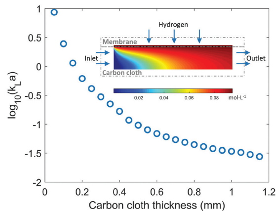
Fig. 3 The mass transfer coefficient k_L a values under various carbon cloth thicknesses. Insert figure: the hydrogen concentration profile in the membrane and carbon cloth (membrane thickness is 40 μm, and carbon cloth thickness is 0.6 mm).
