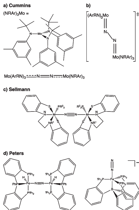
Fig. 2 Thermal dinitrogen activation complexes: (a) Cummins, (b) zig-zag transition state relevant to the Cummins complex, (c) Sellmann, (d) Peters: left [P_2^{PPh}FeH]_2(\mu-N_2) , right [P_3^{BFe}(N_2)]^- .
