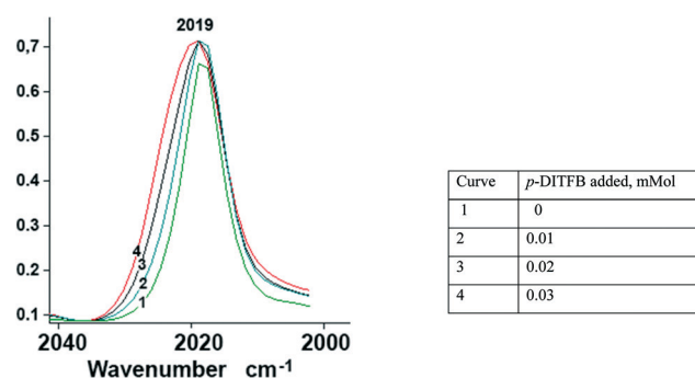
Fig. 1 Unsymmetrical hypsochromic broadening (ca. \sim 4\text{ cm}^{-1} half-width) of the \nu(\text{CO}) band at 2019\text{ cm}^{-1} as a result of gradual addition of p -DITFB to a 0.025 mmol cyclohexane solution of \text{CpFe}(\text{CO})_2\text{TePh} .
