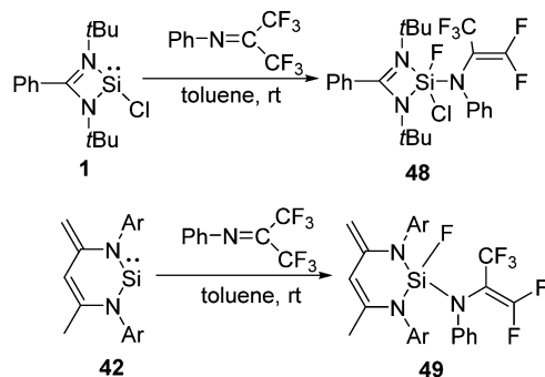
Scheme 17 Activation of the C–F bond in \text{PhC}\equiv\text{N}(\text{CF}_3)_2 by 1 and 42 .
