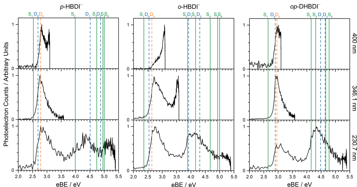
Fig. 2 Photoelectron spectra of p -HBDI ^- (left) o -HBDI ^- (centre) and op -DHBDI ^- (right) recorded at 400 nm (3.10 eV), 346.1 nm (3.582 eV) and 230.7 nm (5.374 eV). Individual spectra have been normalised to their maximum intensity. Vertical dashed orange and blue lines mark the first three vertical detachment energies, calculated using the EPT/6-311++G(3df,3pd) and EOM-IP-CCSD/aug-cc-pVDZ methods, respectively. Vertical green lines mark the VEEs of the anions calculated using the ADC(2)/aug-cc-pVDZ method (solid green).
