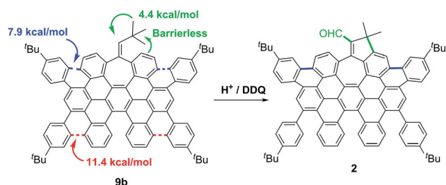
Scheme 3 Summary of calculated energies of subsequent transformations of 9b upon protonation.
