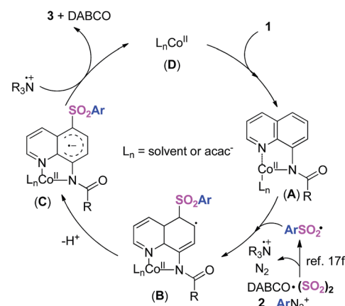
Scheme 5 Plausible mechanism.
