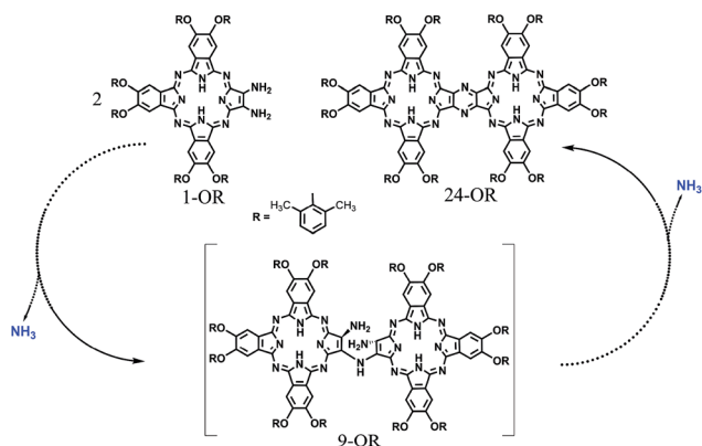
Scheme 3 Schematic of the reaction pathway of the formation of 24-OR with 1-OR as the starting reagent through 9-OR together with the formation of ammonia.
