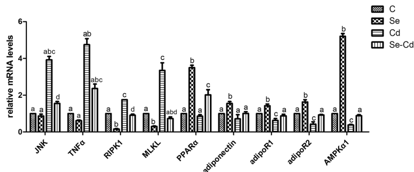
Fig. 5 Effects of four groups C, Se + , Cd + , Se + + Cd + on the mRNA levels of JNK, TNFα, RIPK1, MLKL, PPARα, adiponectin, adipoR1, adipoR2 and AMPKα1 genes in cardiomyocytes. The results were calculated from at least three independent experiments. The data are expressed as the means ± SD. The mean value between groups without a shared common letter are significantly different ( p < 0.05 ), n = 3 , using one-way ANOVA.
