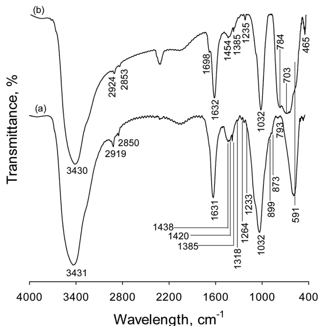
Fig. 4 FT-IR spectra of (a) \text{Fe}_3\text{O}_4 and (b) \text{Fe}_3\text{O}_4@TiO_2 .
