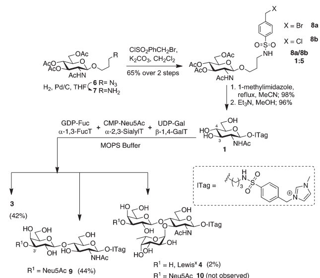
Scheme 1 One-pot in vitro chemo-enzymatic synthesis of ITagged human milk oligosaccharides 3 , 4 and 9 . See ESI† for traces.
