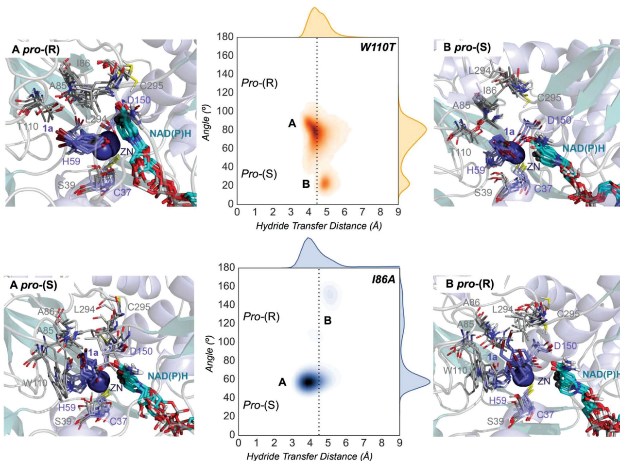
Fig. 4 Representation of some representative snapshots of the different conformational states sampled along the MD simulations for the TbSADH W110T and TbSADH I86A starting from the pro-(R) (in orange) and pro-(S) (in blue) orientations of 1a , respectively. The histogram of the hydride transfer distance together with the pro-(R)/pro-(S) angle (detailed in Fig. S1†) is displayed for both variants.
