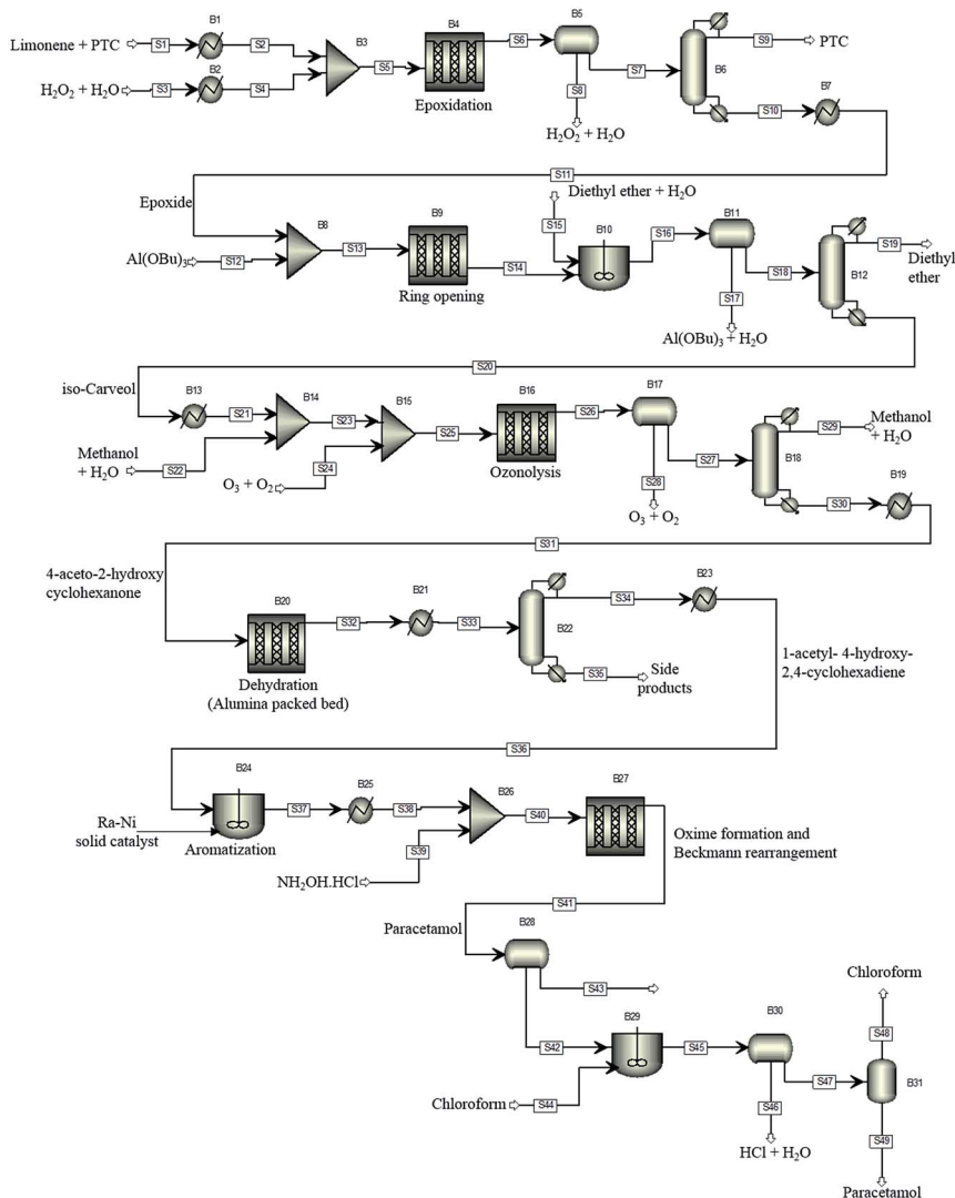
Fig. 4 The proposed process flowsheet detailing all reaction and separation steps. The ASPEN flowsheet is shown for illustration only. All simulations were performed using qPROMS.
