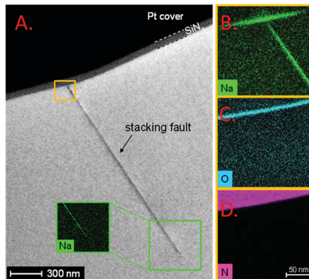
Fig. 5 (A) A bright-field TEM image of a stacking fault representing a single PID-shunt. (B–D) EDX mappings acquired in the STEM mode at the same stacking fault near the interface between Si and Si x N x . A Na-EDX map of the lower part of the stacking fault is also shown in the inset of A. Reprint from ref. 65. Copyright 2014, Elsevier.
