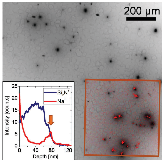
Fig. 4 An EBIC image of a monocrystalline silicon cell region with a high density of PID shunts acquired at an acceleration voltage of 30 kV. The inset shows the distribution of Na at the Si x N x /Si interface measured by the ToF-SIMS. Reprint from ref. 65. Copyright 2014, Elsevier.
