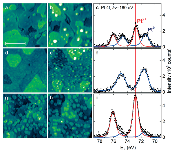
Fig. 14 STM images (a and b, d–e and g–h) and Pt 4f spectra (c, f and i) obtained from the stepped CeO 2 (111) surfaces with a low density of surface oxygen vacancies and steps (a–c), a high density of surface oxygen vacancies (d–f), and a high density of steps (g–i) before (a, d and g) and after (b, e and h) Pt deposition in UHV followed by annealing to 700 K. The size of the images is 45 × 45 nm 2 and the scale bar is 20 nm. All STM images were obtained with a tunneling current of 25–75 pA and a sample bias voltage of 2.5–3.5 V. Pt 4f spectra were acquired with photon energy h\nu = 180 eV. Reproduced with permission from ref. 22, Copyright 2016, Nature Publishing Group.
