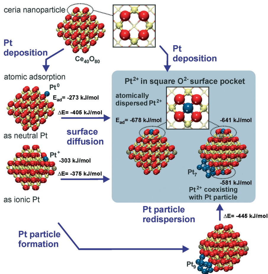
Fig. 6 Structure and energetics of various anchored Pt species on ceria nanoparticles obtained from density functional calculations. Pt 2+ is strongly bound to square O 4 pockets at the {100} nanofacets of the particles. Color coding of atoms: red O, beige Ce 4+ , brown Ce 3+ , and blue Pt. Reproduced with permission from ref. 70, Copyright 2016, Springer International Publishing AG.
