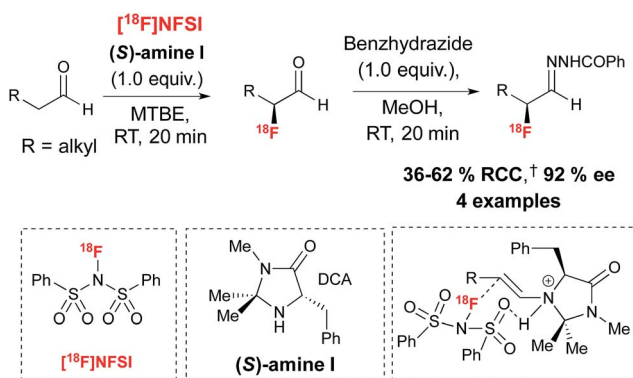
Scheme 5 Chiral imidazolidinone ( S )-I for the enantioselective ^{18}\text{F} -fluorination of aldehydes with ^{18}\text{F} -NFSI. †RCC determined by radio-HPLC relative to ^{18}\text{F} -NFSI. DCA = dichloroacetic acid. For ^{18}\text{F} -NFSI, SA = 0.05 \text{C}_i \mu\text{mol}^{-1} , ( n = 3 ).
