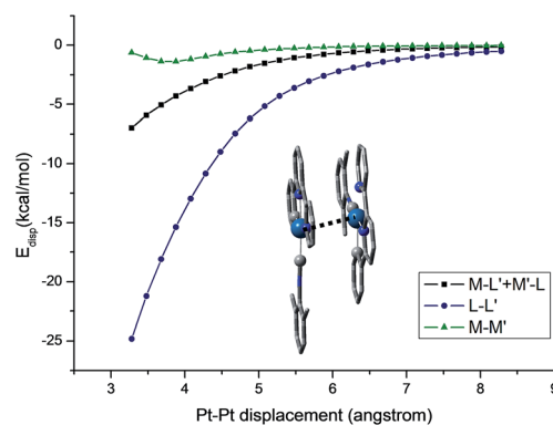
Fig. 13 Dispersion contributions of the metal atoms and ligand fragments to the dimer [61-PF 6 ] 2 2+ . The Pt...Pt distance was used as a reaction coordinate.
