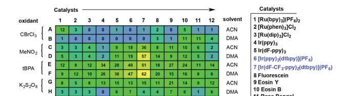
Fig. 2 Identification of a photoredox-mediated dehydrogenation via high-throughput experimentation. Reactions performed on 2.5 \mu mol scale using 465 nm LEDs. Numbers in table refer to assay yields based on HPLC analysis with an internal standard.
