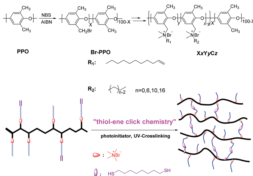
Scheme 1 Synthesis of cross-linked comb-shaped AEMs, XxYyCz , with one alkyl side chain using thiol–ene click chemistry.
