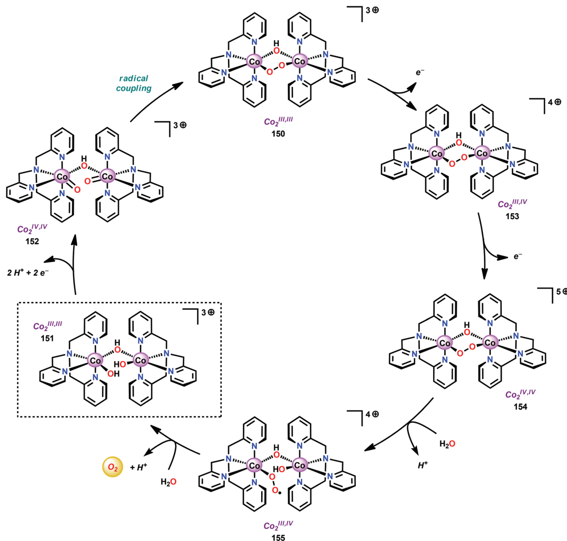
Scheme 10 Proposed mechanism for \text{H}_2\text{O} oxidation catalyzed by the dinuclear [(\text{tpa})\text{Co}(\mu\text{-OH})(\mu\text{-O}_2)\text{Co}(\text{tpa})]^{3+} complex 150. tpa = tris(2-pyridyl-methyl)amine.
