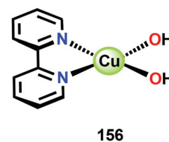
Fig. 51 Structure of the [\text{Cu}(\text{bpy})(\text{OH})_2] complex 156.
