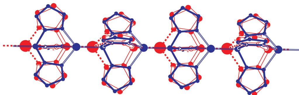
Fig. 8 Disorder in the one-dimensional Cu coordination chain of [(C^H Cu)(PF_6)]_n . Location in the unit cell at (2/3, 1/3, z) , Wyckoff position b . The major disorder component is drawn in red, the minor component in blue. The estimated ratio between the two components is 65 : 35%.
