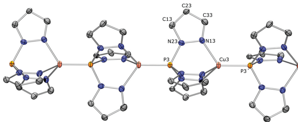
Fig. 7 One-dimensional Cu coordination chain in the crystallographic c -direction of [(C^H Cu)(PF_6)]_n . Only one of the two independent polymers is shown. Location in the unit cell at (0, 0, z) , Wyckoff position a . A slight disorder in this chain has been ignored in the structure refinement. In the drawing, hydrogen atoms, PF_6 anions and C_2H_4Cl_2 solvent molecules have been omitted for clarity. Symmetry codes: (i) y, x, z - 1/2 ; (ii) y, x, z + 1/2 ; (iii) x, y, z + 1 . Selected bond lengths [Å] and angles [°]: Cu3–N13 2.034(5), Cu3–P3' 2.081(2), P3–N23 1.700(4), P3...Cu3 3.227(2), N13–Cu3–N13 93.22(17), P3'–Cu3–N13 122.95(12), N23–P3–N23' 101.8(2).
