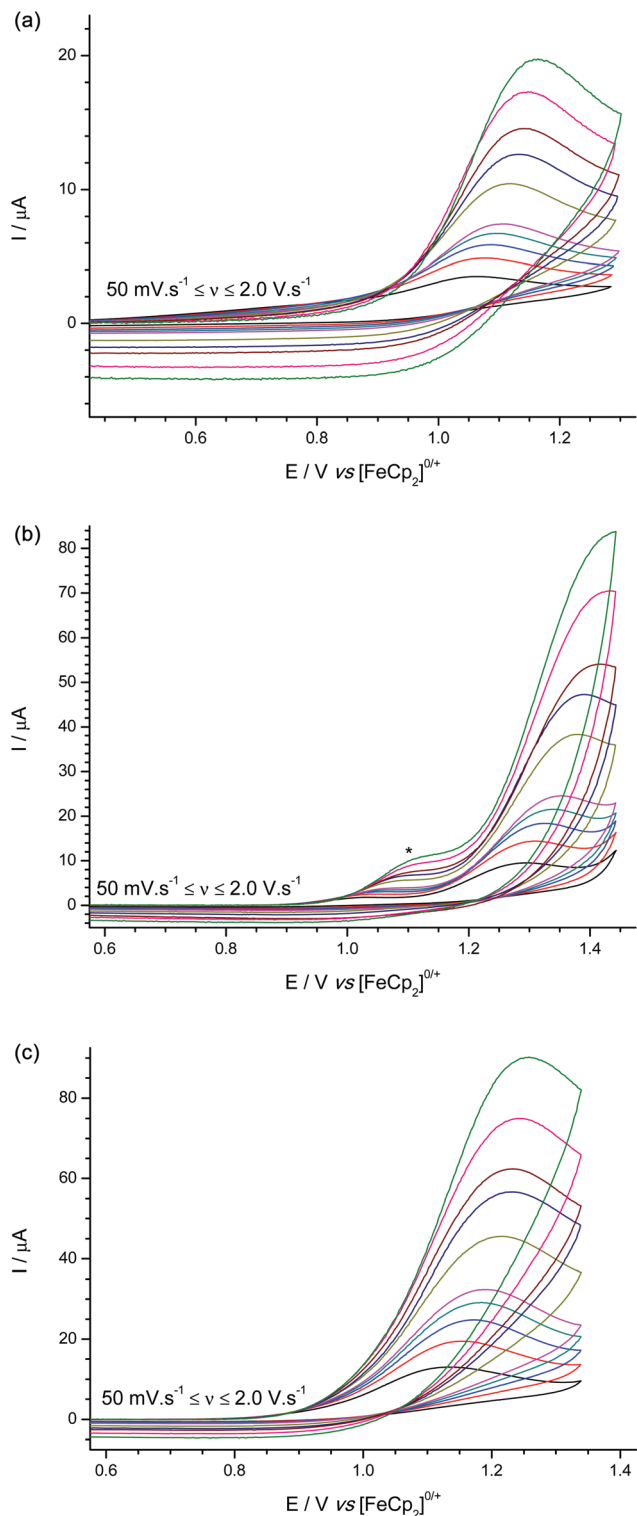
Fig. 5 Experimental cyclic voltammograms for the oxidation of (a) \text{Na}[1\text{-H}] , (b) \text{Na}[2\text{-H}] , and (c) \text{Na}[3\text{-H}] shoulder (*) visible at the higher scan rates due to trace impurity in the solvent/electrolyte.
