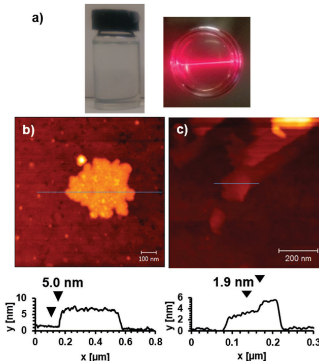
Fig. 2 (a) Images showing a suspension of Cu(1) nanosheets in DMF with characteristic Tyndal Scattering of laser light. AFM images and height profiles corresponding to blue lines for nanosheets formed by exfoliation of (b) Zn(1) in DMF (c) Cu(1) in H_2O .
