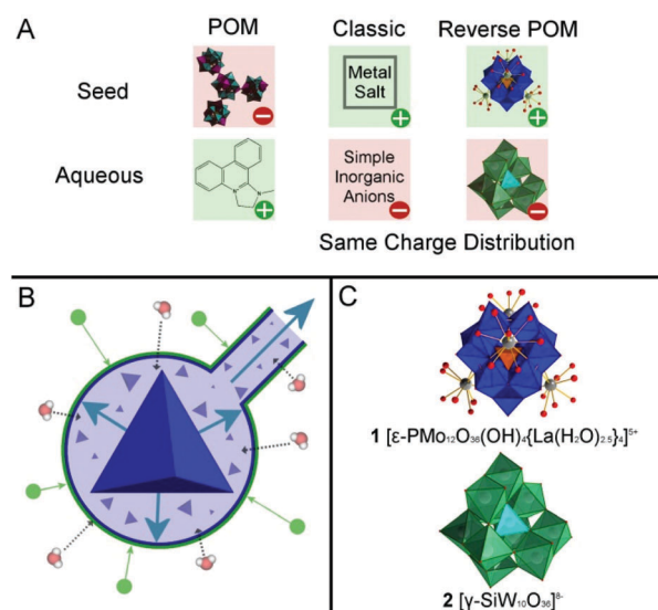
Fig. 1 (A) A graphical representation of some different types of chemical gardens that are known; previously reported POM chemical gardens, classic chemical gardens and the charge reversed POM chemical gardens presented herein. (B) A schematic representation of the general POM chemical garden growth mechanism. (C) Structures of the POMs used in this study. Blue – Mo, Orange – P, Grey – La, Red – O, Green – W, Teal – Si.
