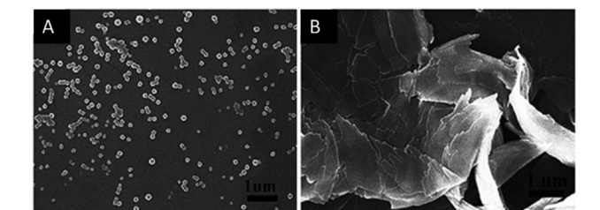
Fig. 34 Schematic representation of the anion- \pi induced self-assembly forming the vesicle as well as SEM images before (A) and after addition of 3 eq. of NaNO 3 (B). Reproduced with permission from John Wiley and Sons. 66
