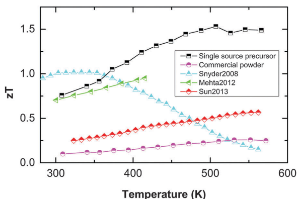
Fig. 5 Compilation of Sb 2 Te 3 figure of merit data, comparing own data (single-source precursor material and commercial powder processed identically) with literature references: nanostructured Sb 2 Te 3 shows best zT values around 0.6 (Sun 2013 23 ). Co-doping the nanomaterial electrically with sulphur raises zT up to 1 (Mehta 2012 24 ). zT values around 1 were presented in the review of Snyder and Toberer for commercial Sb 2 Te 3 , without further elaboration on the material's chemistry or preparation route (Snyder 2008 25 ).
