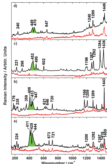
Fig. 10 Resonance Raman ( \lambda_{\text{exc}} = 647 nm) of 3 (a), 4 (b), 5 (c), 6 (d) at 300 K (red lines), 20 K (black lines) and electronic transition coloured in green.
