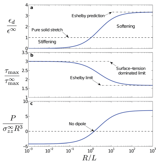
Fig. 3 Liquid inclusion characteristics as a function of size R/L for inclusions in an incompressible solid with an applied uniaxial far-field stress as shown in Fig. 1 (a) Droplet strain, \epsilon_d = (\ell - 2R)/R divided by far-field strain \epsilon^\infty only depends on R/L . When R/L \ll 1 , surface tension dominates and there is no droplet deformation. When R/L \gg 1 , surface tension is negligible and the shape prediction is that of classical Eshelby theory – given by the dash-dotted line. The dashed line shows the material stretch, (\ell - 2R)/R = \epsilon^\infty . (b) The shear-stress concentration factor at the inclusion tip ( r = R , \theta = 0 ). This corresponds to the highest shear stress in the solid around the inclusion (see Fig. 2, bottom row). Dash-dotted lines show surface-tension dominated and Eshelby limits: \tau_{\max}/\tau_{\max}^\infty = 3 , 5/3 respectively. (c) The far-field dipole caused around the inclusion. Note that this dipole changes sign at R = 1.5L , indicating the transition between inclusion stiffening and inclusion softening of the composite.
