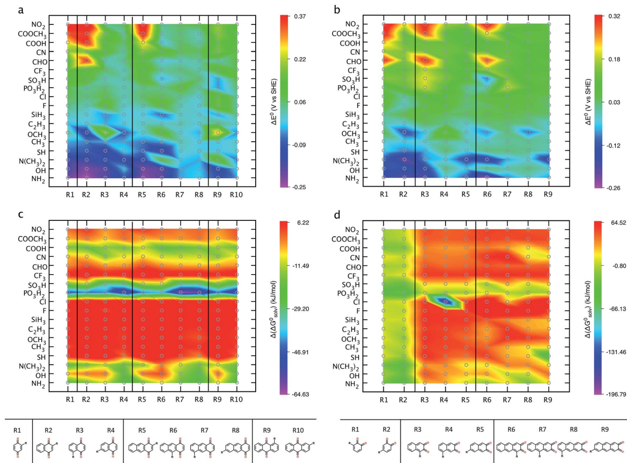
Fig. 6 Positional effects of R-groups on the E^\circ and \Delta G_{\text{solv}}^\circ . (a and c) Show the results for the single R-group functionalized para -(BQ, NQs, and AQs), whereas (b and d) show the results for the single R-group functionalized ortho -(BQs, NQs, and AQs).
