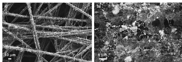
Fig. 5 SEM images of electrosprayed 46 wt% Pt-CNT–CsH 2 PO 4 composites, showing direct contact between the electrolyte particles with the carbon nanotubes: (a) low and (b) high magnification.
